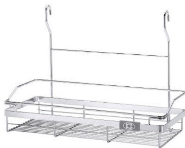
HC-3025-1200 單層置物架 Multipurpose Rack L400 x W185 x H300 mm
